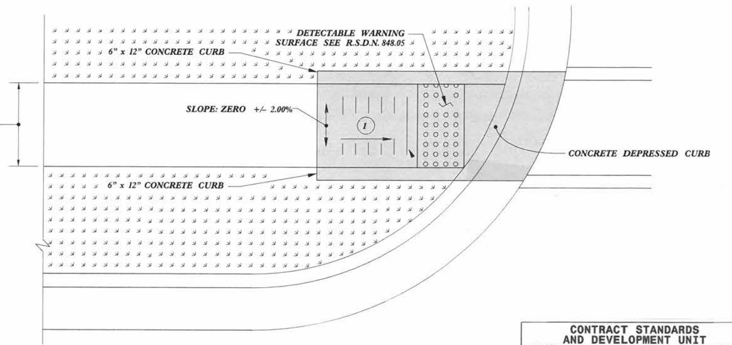
TYPE 1 Modified
